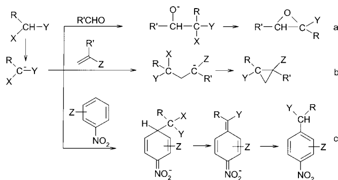
Scheme 1. Typical reactions of \alpha -halocarbanions.
