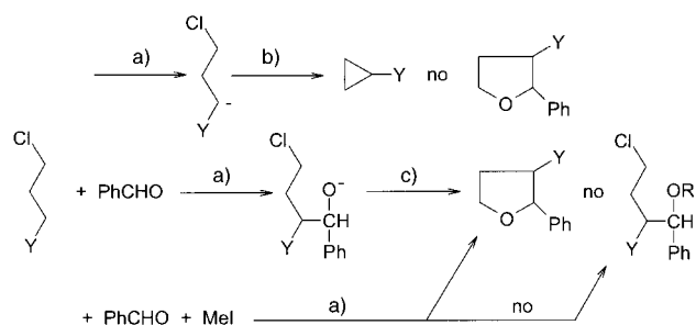
Scheme 3. Competition between intermolecular and intramolecular reactions in THF solutions. a) t BuOK, -70^{\circ}\text{C} ; b) PhCHO, c) MeI or \text{Me}_3\text{SiCl} .
