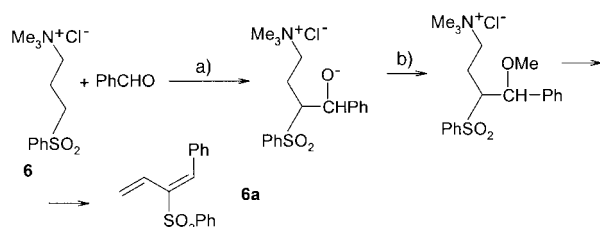
Scheme 6. Reaction of the carbanion of 3-trimethylammoniopropyl phenyl sulfone with benzaldehyde and methyl iodide. a) t BuOK, b) MeI.
