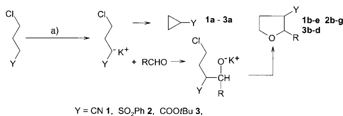
Scheme 2. Synthesis of cyclopropanes and tetrahydrofurans through intramolecular and intermolecular reactions of \gamma -chlorocarbanions. a) t BuOK, -30^\circ\text{C} , 0.5 M solution of 1 , 2 , 3 in THF.
